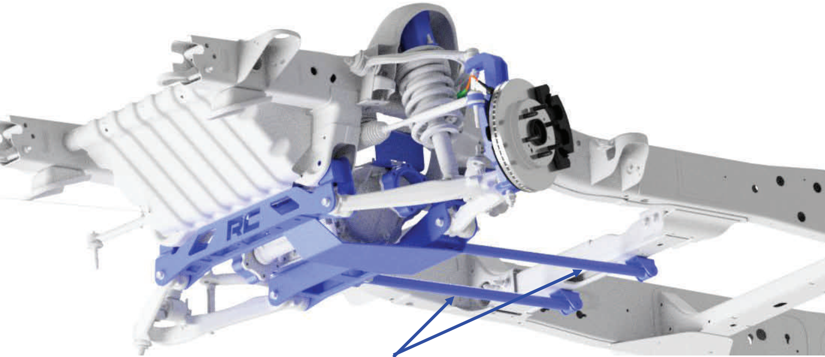
DIAGRAM SHOWN WITH OPTIONAL KICKER BARS PART #1262 INSTALLED
