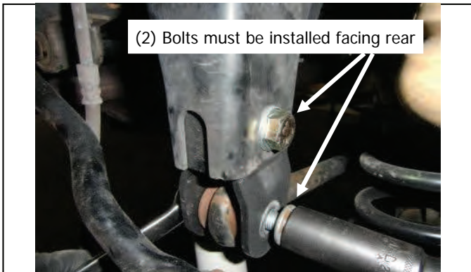
Carefully raise rear axle to reinstall OE upper trac bar bolt
