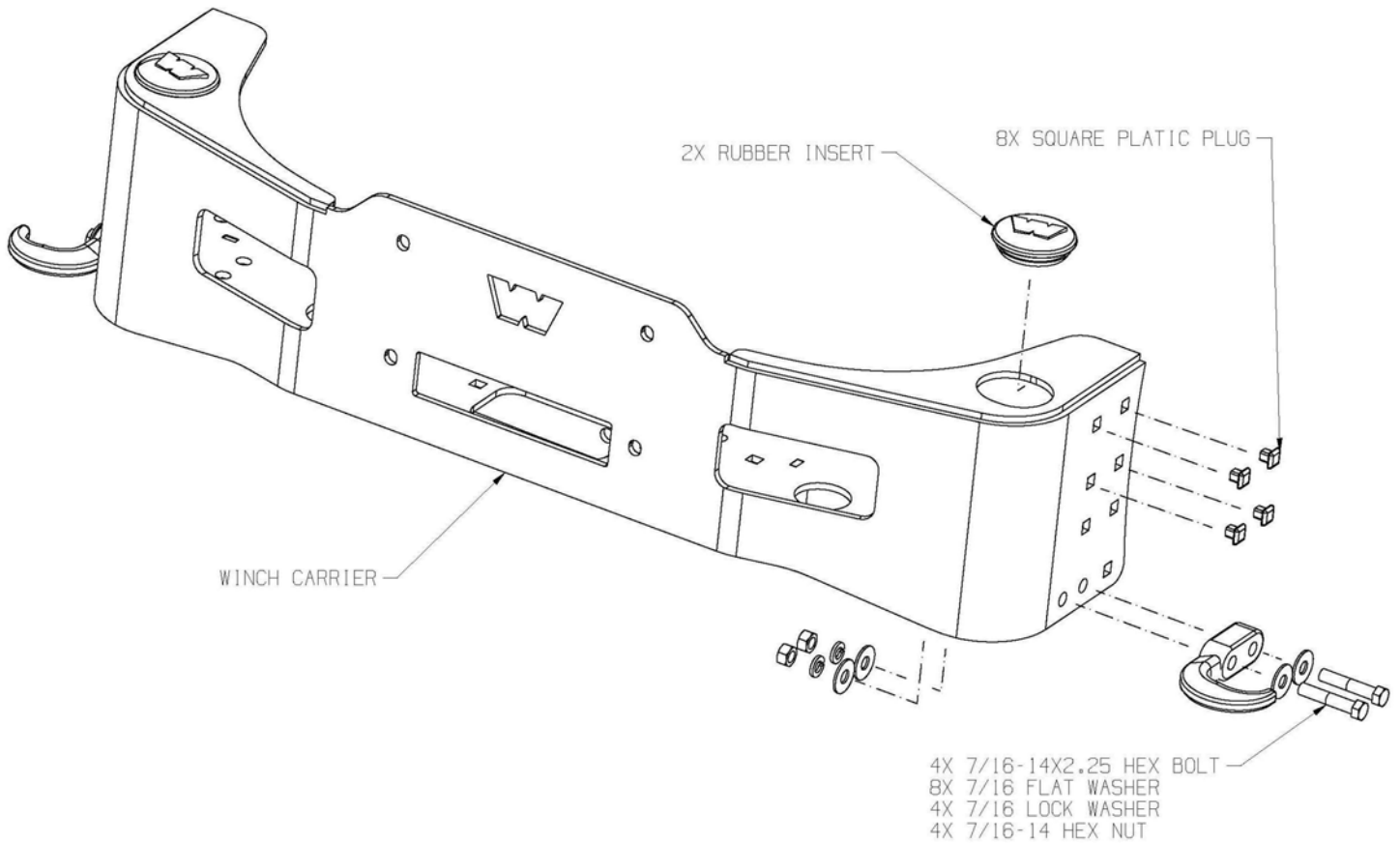
Figure A: Large Frame Exploded View
