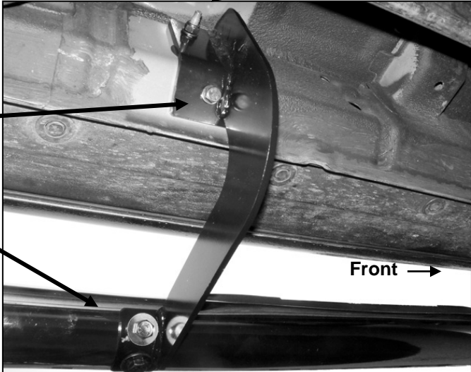
(Fig 4) Driver side center mounting location pictured
