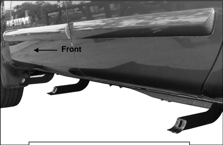
(Fig 3) Driver side Brackets installed. Note all cradles face back of vehicle
