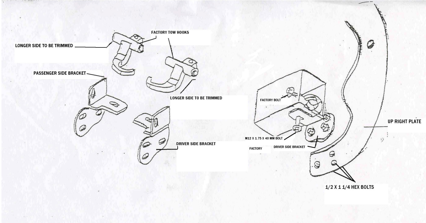
ILLUSTRATION 3- TOP BRACKETS
