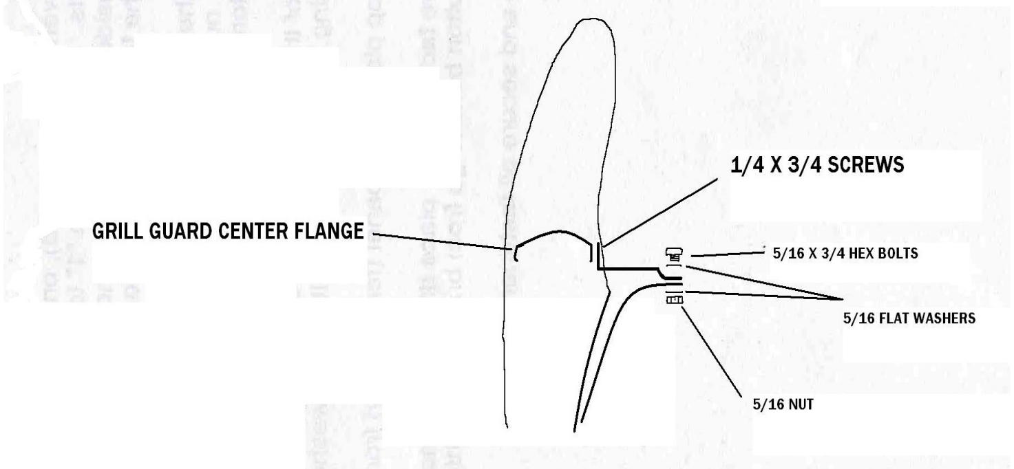
ILLUSTRATION 3- TOP BRACKETS
