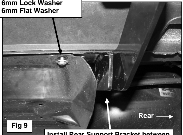
Install Rear Support Bracket between plastic cover and frame channel
